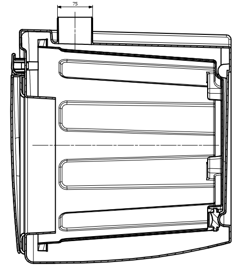
SECTION E-E
